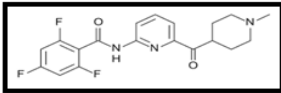
Fig 1: Molecular structure of Lasmiditan
